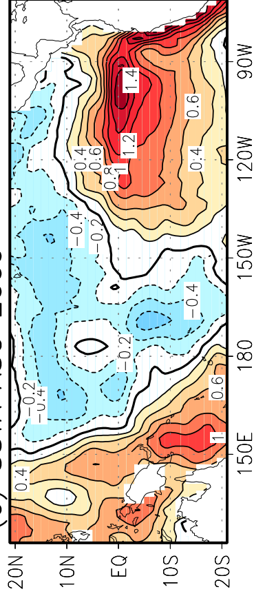
(c) SSTA ASO 2009
