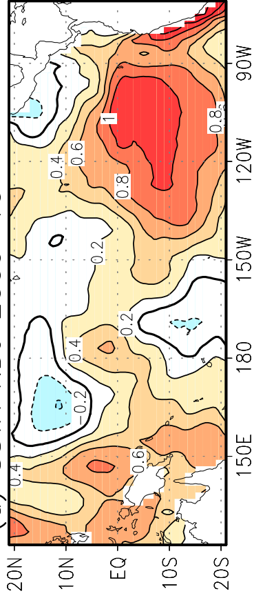
(a) SSTA NDJ 2009–10
